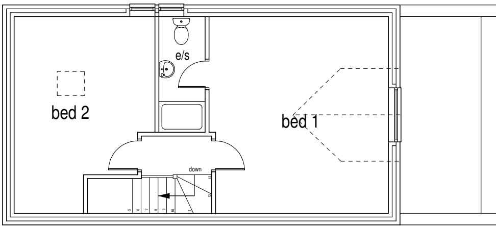
Second floor layout.
